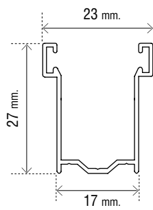
Art. OMTGU1728 Guida in alluminio 17 x 27 mm.
