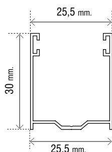
OMTGU2530
