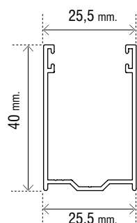
Art. OMTGU2540
