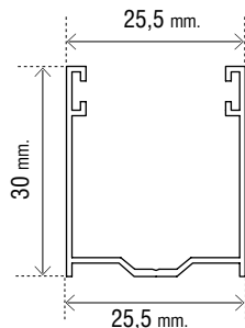
Art. OMTGU2530
