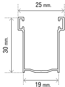
Art. OMTGU1928 Guida in alluminio 19 x 30 mm.
