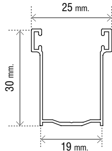
Art. OMTGU1928
