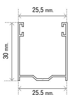
Art. OMTGU2530
