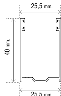
Art. OMTGU2540 Guida in alluminio 25,5 x 40 mm.
