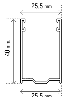
Art. OMTGU2540
