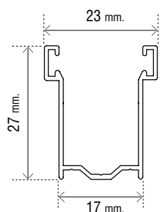
Art. OMTGU1728 Guida in alluminio 17 x 27 mm.
