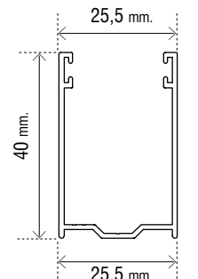
Art. OMTGU2540
