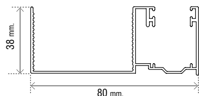
Art. OMTGU8038
