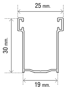
Art. OMTGU1928
