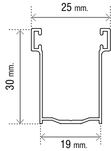
Art. OMTGU1928 Guida in alluminio 19 x 30 mm.
