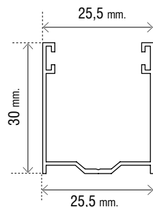
Art. OMTGU2530
