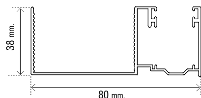
Art. OMTGU8038
