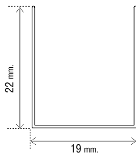
Art. OMTGUFEZI
