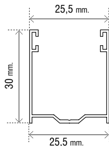
Art. OMTGU2530 Guida in alluminio 25,5 x 30 mm.
