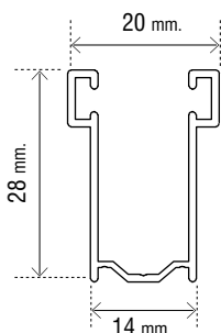
Art. OMTGU1428 Guida in alluminio 14 x 28 mm.
