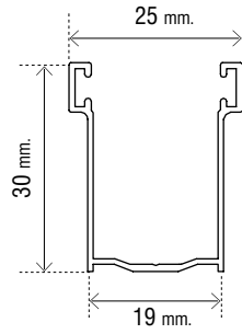
Art. OMTGU1928 Guida in alluminio 19 x 30 mm.
