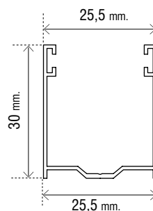
Art. OMTGU2530
