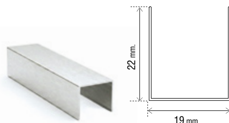
Guida in ferro 19 x 22 mm
