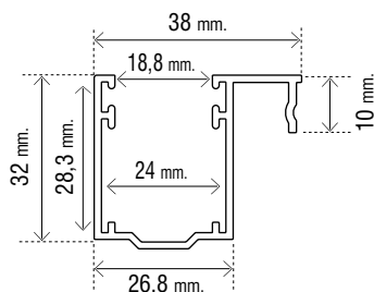
Art. OMTGU3832 Guida in alluminio 38 x 32 mm.
