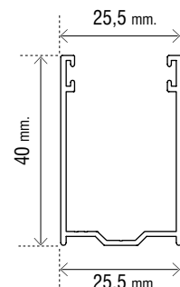
Art. OMTGU2540 Guida in alluminio 25,5 x 40 mm.
