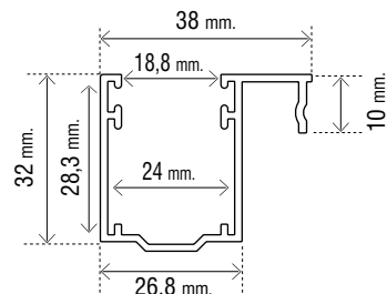
Art. OMTGU3832
