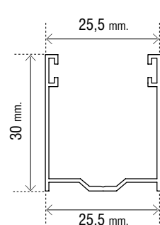
Art. OMTGU2530 Guida in alluminio 25,5 x 30 mm.
