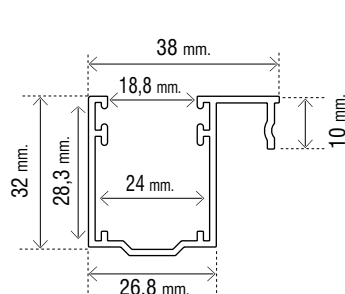
Art. OMTGU3832
