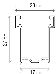
Art. OMTGU1728
