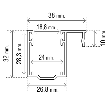
Art. OMTGU3832 Guida in alluminio 38 x 32 mm.
