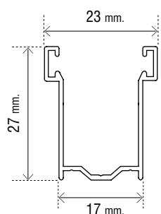
Art. OMTGU1728
