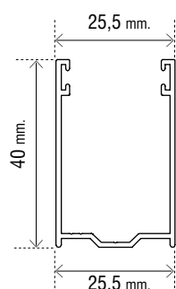
Art. OMTGU2540
