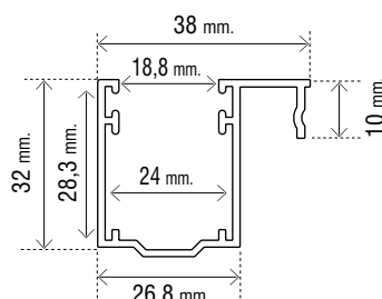
Art. OMTGU3832
