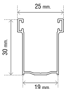
Art. OMTGU1928
